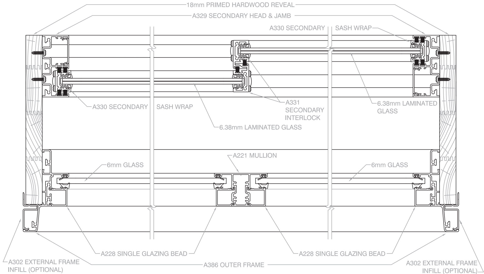
Scale 1 : 2 @ A4, Horizontal Cross Section of Fixed Lite (OO) with secondary glazing (XX)
