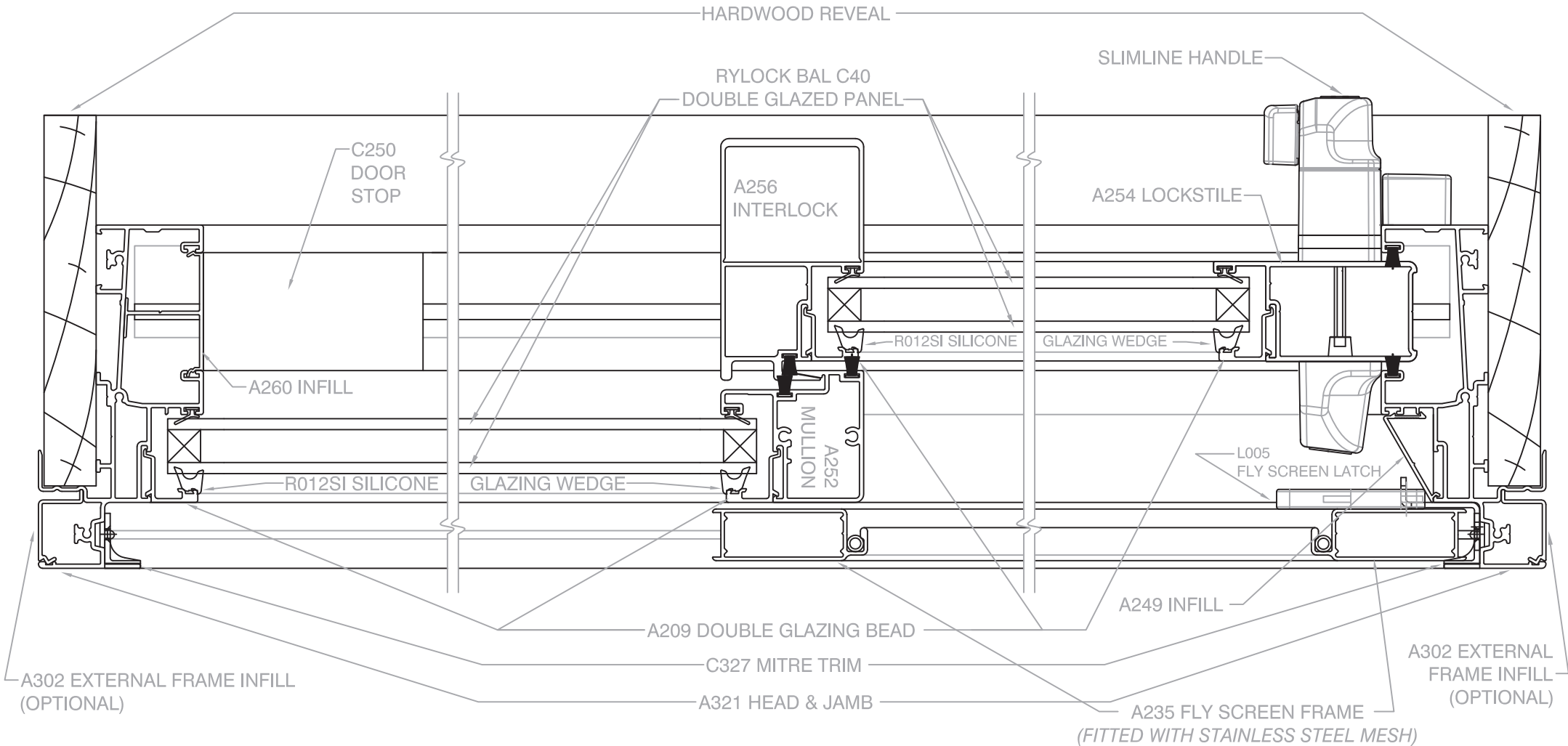
Scale 1 : 2 @ A4, Horizontal Cross Section of 2-Panel Sliding Door (OX)
