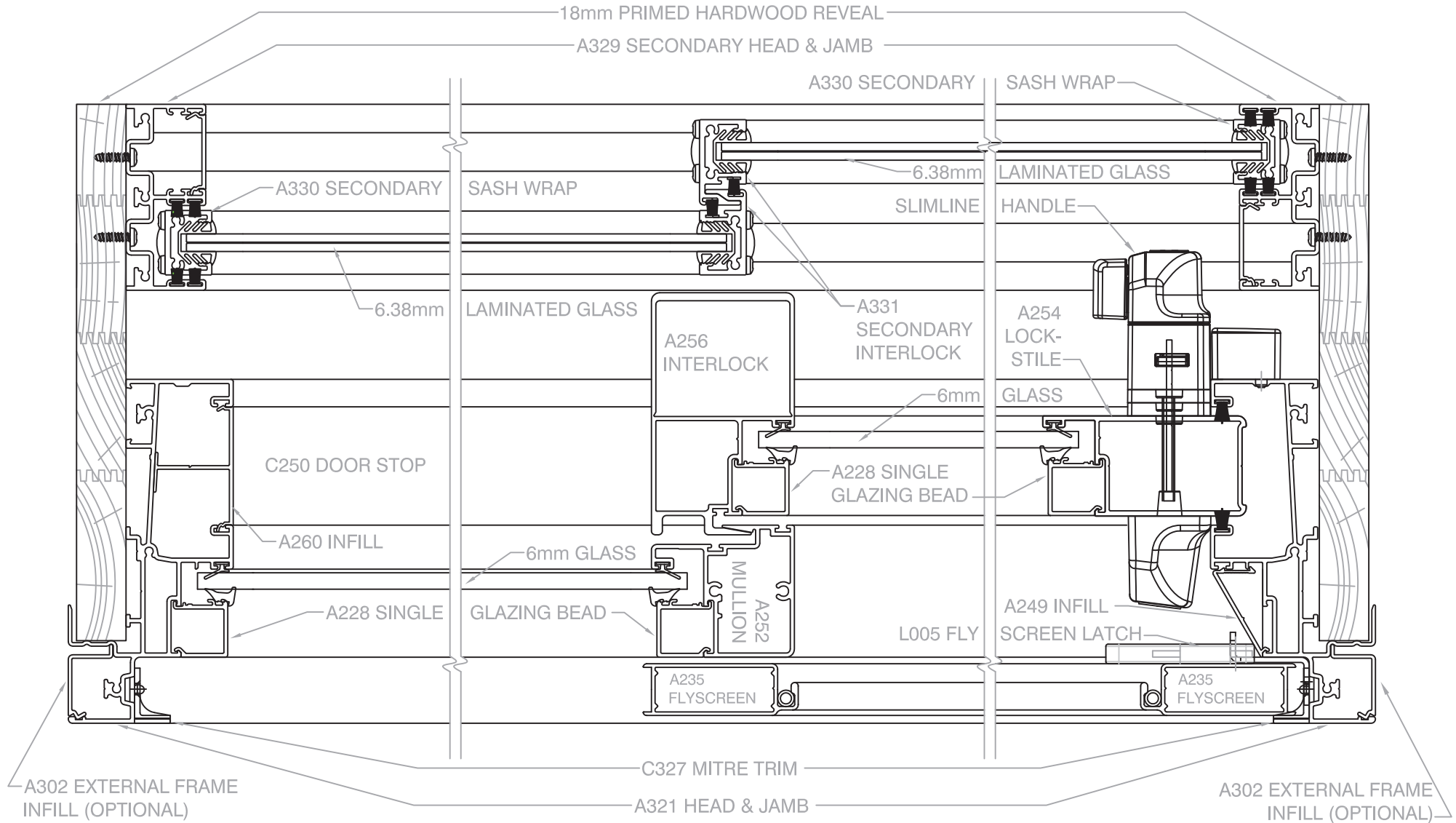
Scale 1 : 2 @ A4, Horizontal Cross Section of 2-Panel Sliding Door (OX) with secondary glazing (XX)
