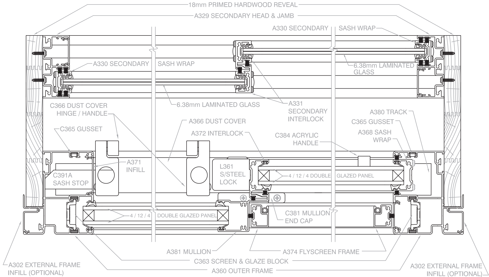
Scale 1 : 2 @ A4, Horizontal Cross Section of 2-Panel Sliding Window (OX) with secondary glazing (XX)
