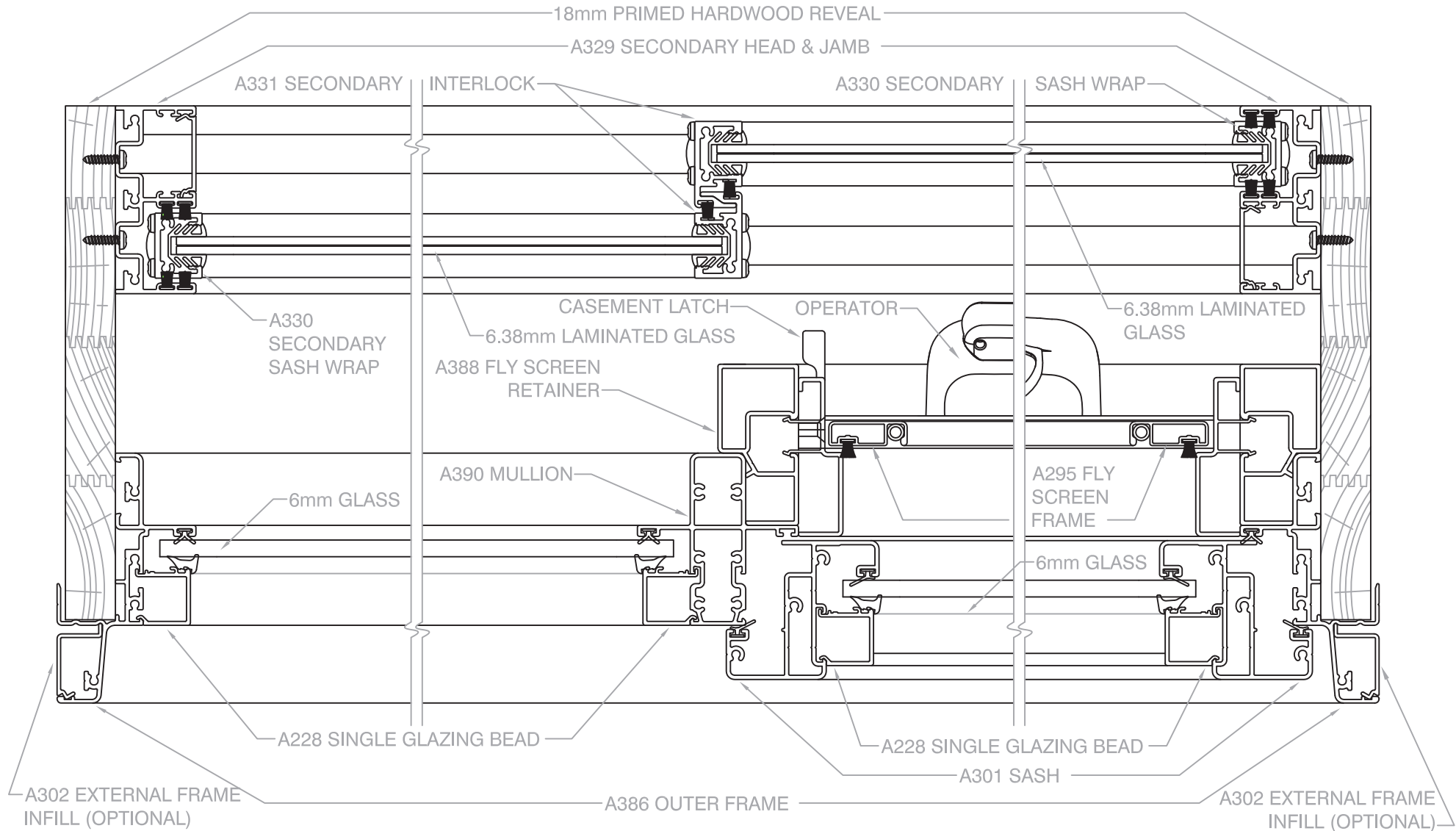
Scale 1 : 2 @ A4, Horizontal Cross Section of Casement next to fixed panel (OV) with secondary glazing (XX)
