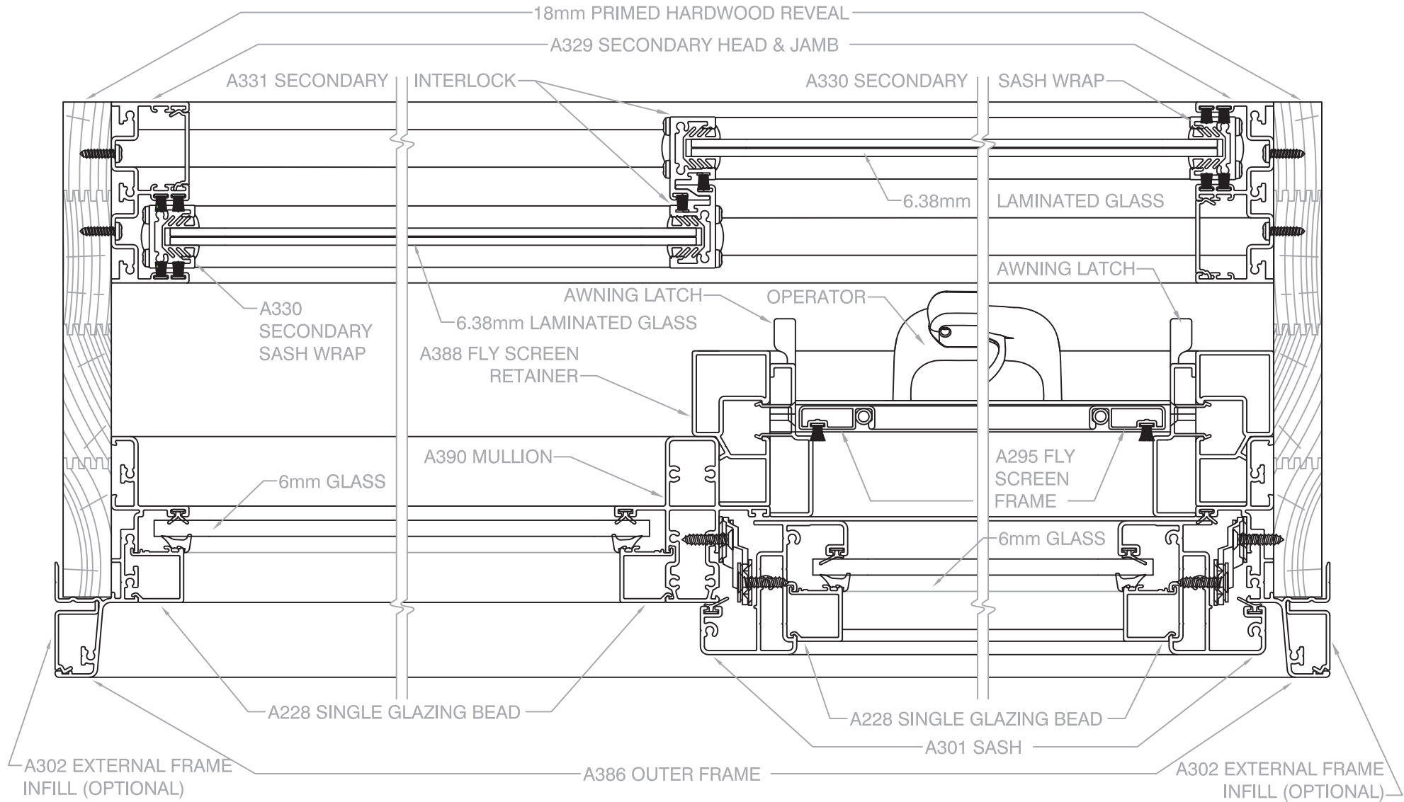
Scale 1 : 2 @ A4, Horizontal Cross Section of Awning next to fixed panel (OV) with secondary glazing (XX)
