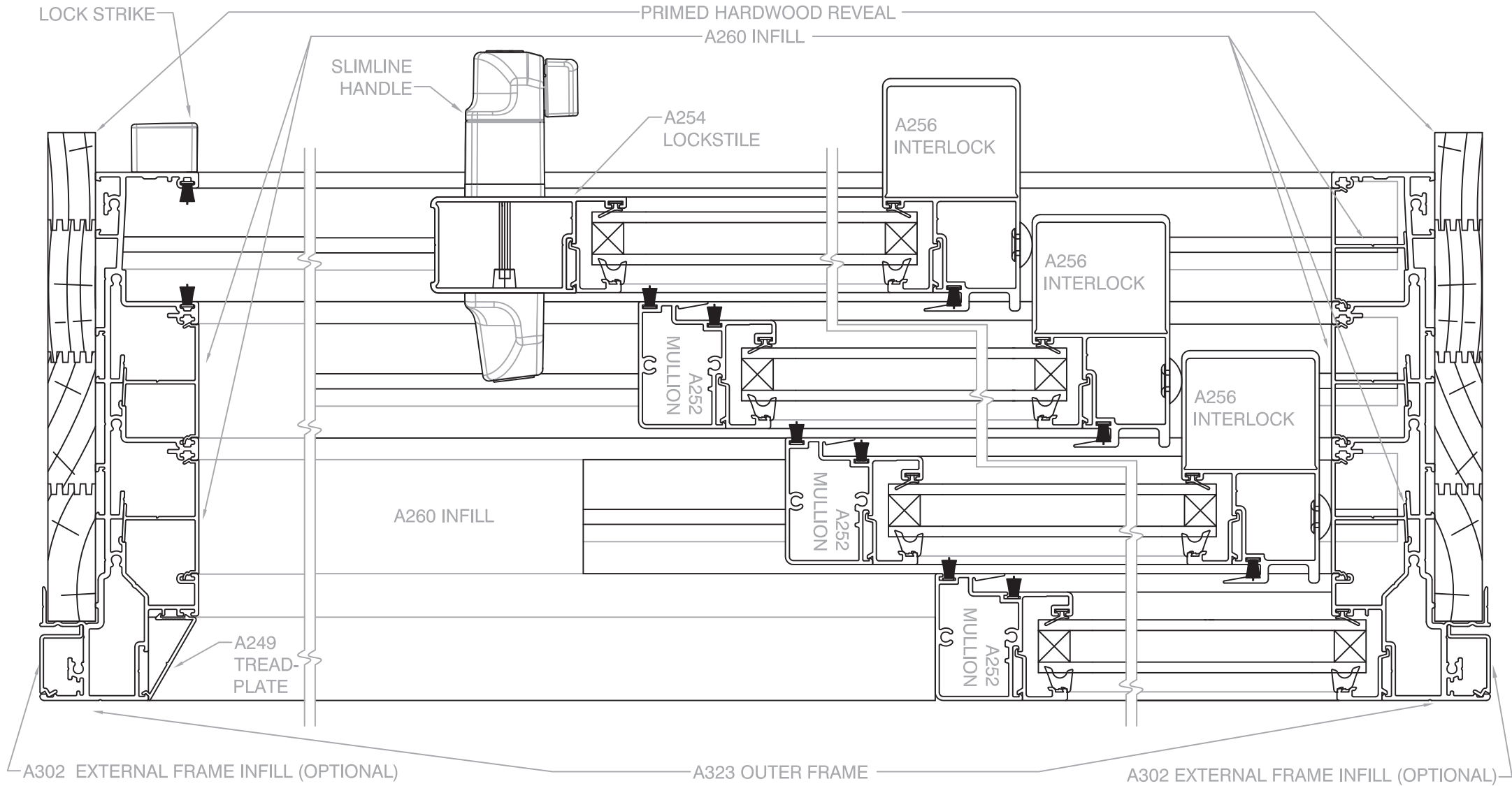
Scale 1 : 2 @ A4, Horizontal Cross Section of 4-Panel Stacker Door
