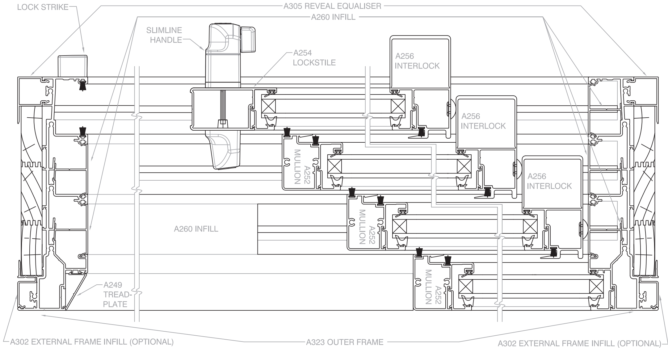
Scale 1 : 2 @ A4, Horizontal Cross Section of 4-Panel Stacker Door, shown with Reveal Equaliser
