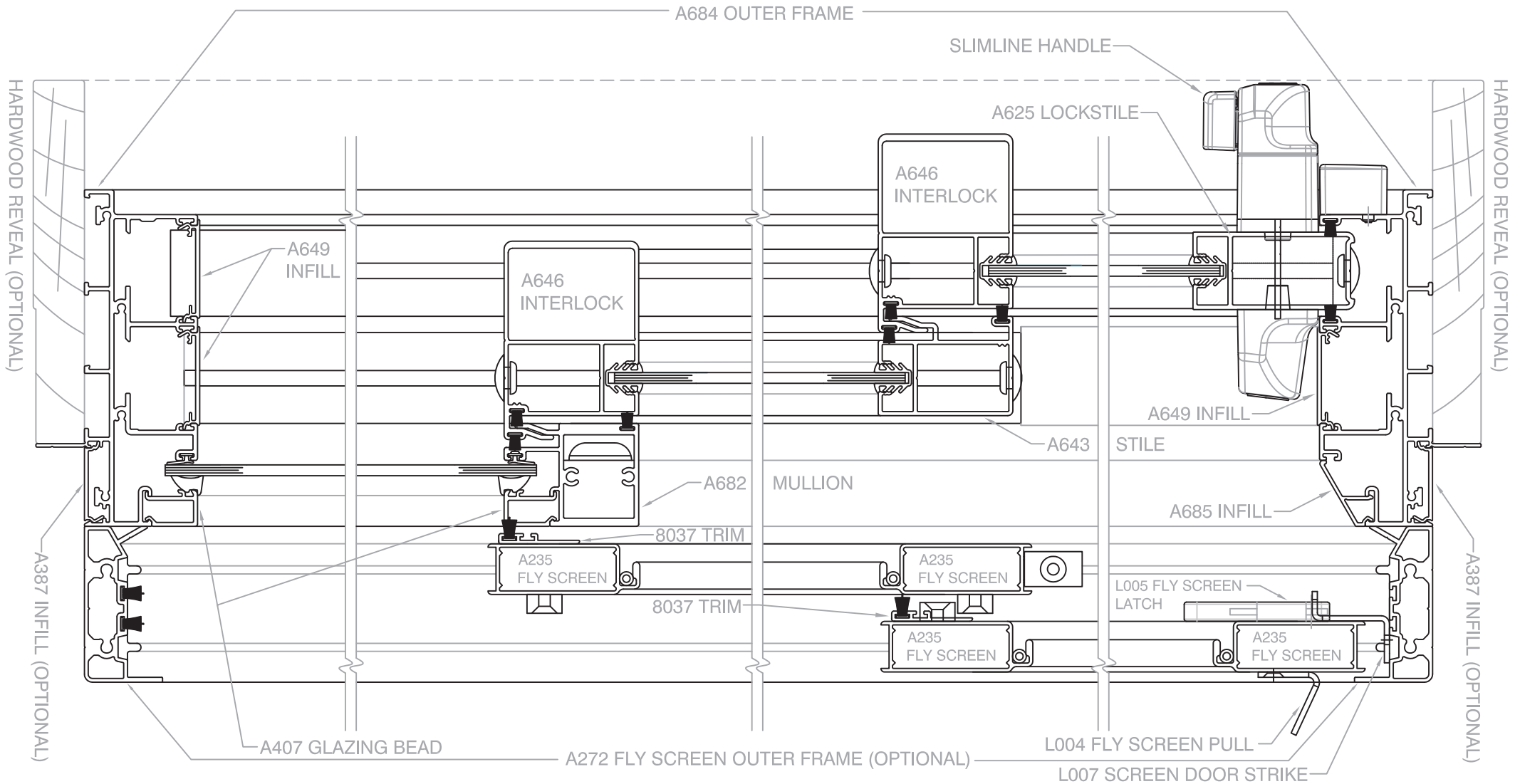
Scale 1 : 2 @ A4, Horizontal Cross Section of 3-Panel Stacker Door (OXX), shown with optional stacking fly screen
